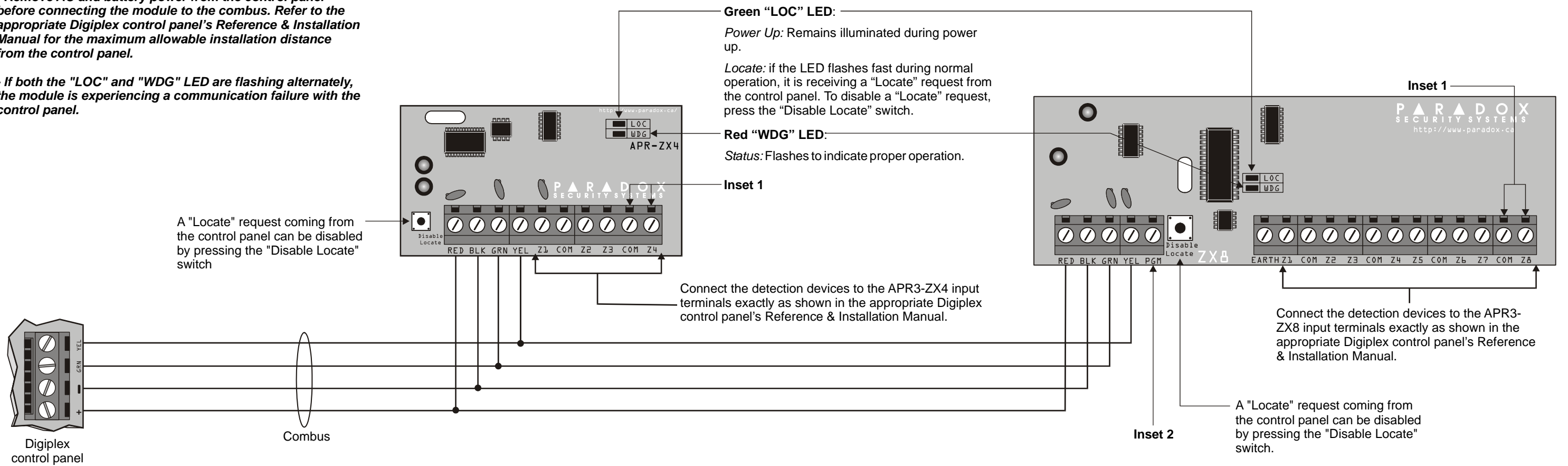
Figure 1: Connecting the APR3-ZX4 and APR3-ZX8
